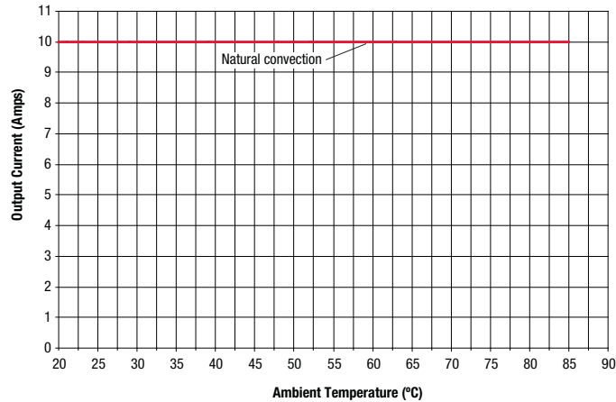
OKY2-T/10-D12-C Maximum Current Temperature Derating at Sea Level (V IN = 12V, V OUT = 0.75 to 5V).
